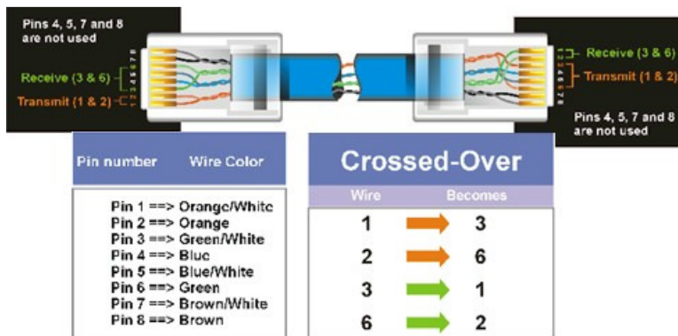
Pinout of crossover-cable
