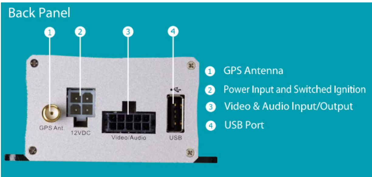
Figure 1-2 Rear Panel
