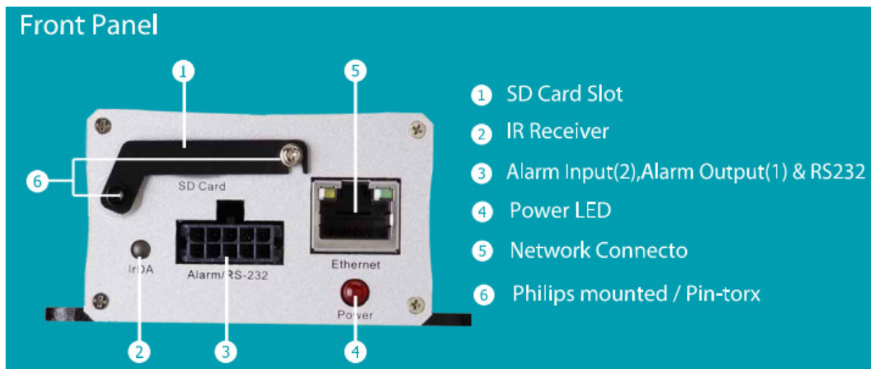
Figure 1-1 Front Panel
